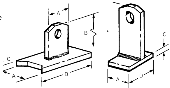
P95P Fleet-Lift Plate Anchor (FL043 only)
