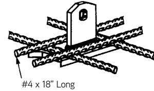
P95P Fleet-Lift Plate Anchor (FL043 only)
