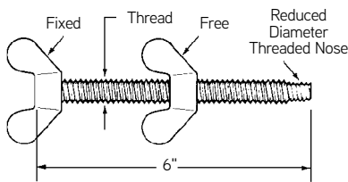
P63PL Swift Lift Plus Holding Stud
