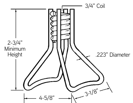
F47 Double Flared Loop Insert
