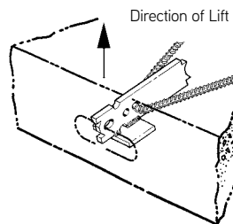
Typical P92HP Fleet-Lift Two-Hole Erection Anchor with Shear Plate Application
