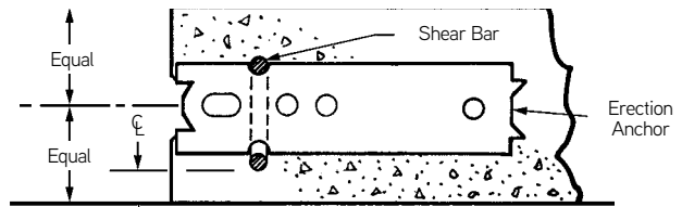
Minimum 3/4" Concrete Cover
