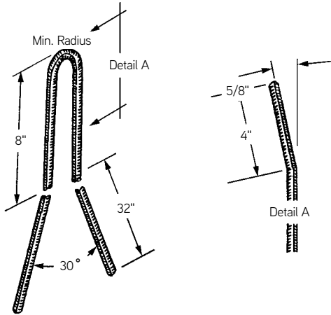
Rebar for 2" x 2" x 2" Panel
