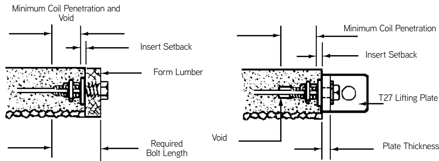
Setting Bolt
