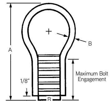
F42 Loop Ferrule Insert
