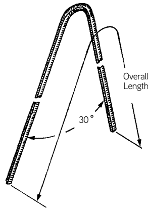
Rebar for 3" x 2" x 3", 2" x 2" x 4", 3" x 3" x 3" and 3" x 4" x 3" Panels
