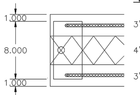
Rebar for 3" x 2" x 3", 2" x 2" x 4", 3" x 3" x 3" and 3" x 4" x 3" Panels
