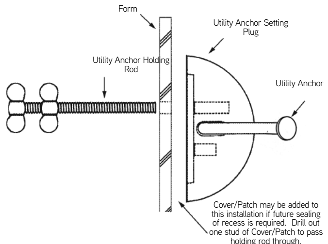
Through-Form Setting
