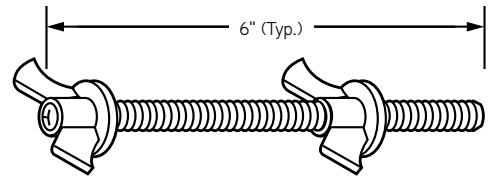
P101 Utility Anchor Holding Rod (3/8" Coil Thread) (FL131)
