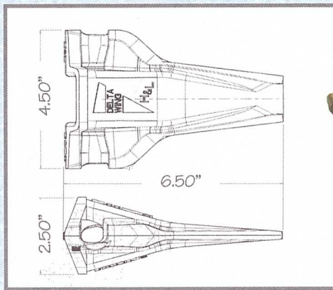
230SP-5 Sharp Penetration 3.2#/1.5kgs
