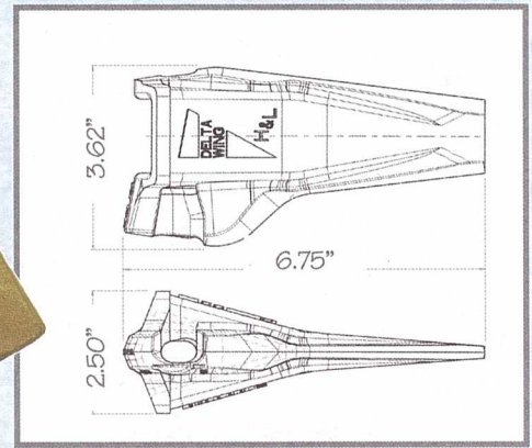
230SP-5C Corner Penetration 2.9#/1.3kgs
