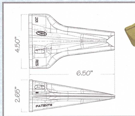
201RE-5 Sharp Penetration 3.3#/1.5kgs
