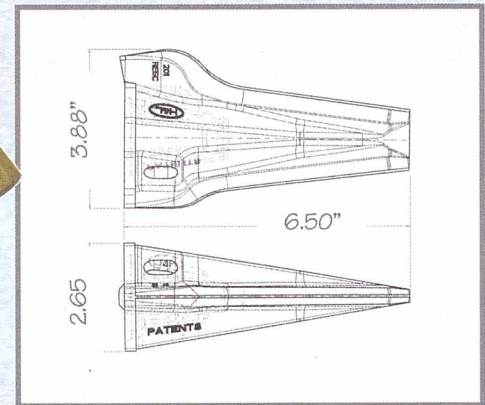
201RE-5C Corner Penetration 3.1#/1.4kgs
